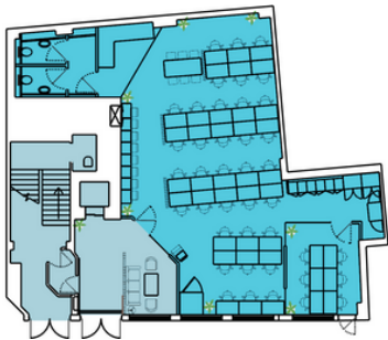
HUBFLOW LAYOUT
